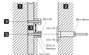
Fig.1 Front-end arrangement maximal axial misalignment \leq 2\text{mm}
